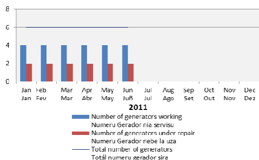
Number of Power Generators in Oecusse Numeru Gerador EDTL iha Oekusi
