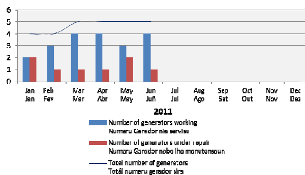
Number of Power Generators in EDTL Ermera Numeru Genarador EDTL iha Ermera
