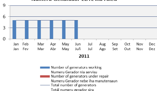
Number of Power Generators in EDTL Aileu Numeru Genarador EDTL iha Aileu
