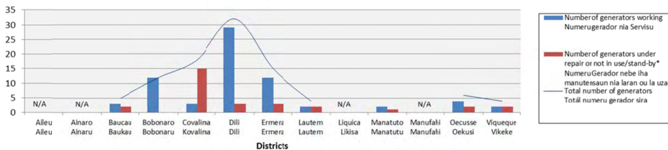
Number of EDTL Generators by Districts in July 2011 Totál Gerador EDTL kada Distritu iha Julu 2011
